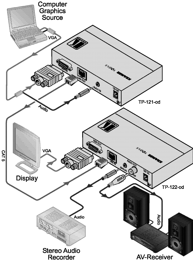
Figure 6: Connecting the TP-121-od and the TP-122-od
