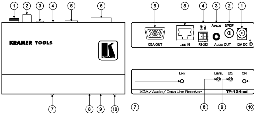
Figure 8: TP-124-od XGA / Audio / Data Line Receiver (Topside)
