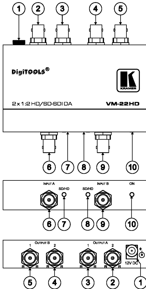
Figure 1: VM-22HD 2 x 1:2 HD/SD-SDI DA
