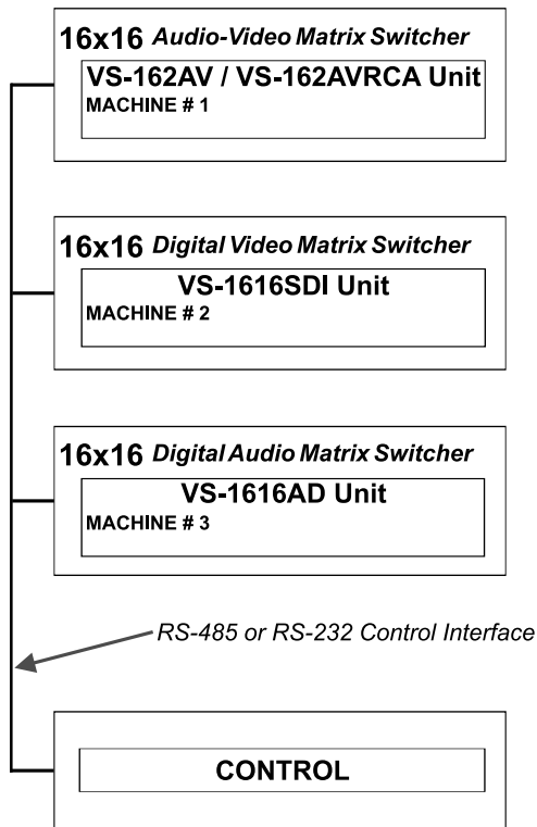
Figure 7: Assembling a System of Interconnected Switchers
